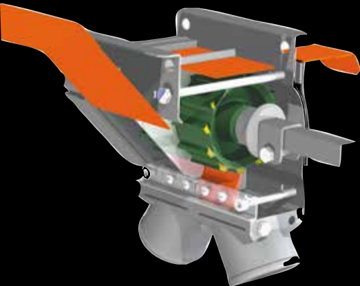
Precise metering by volume through cell wheel metering system with sealing lip
